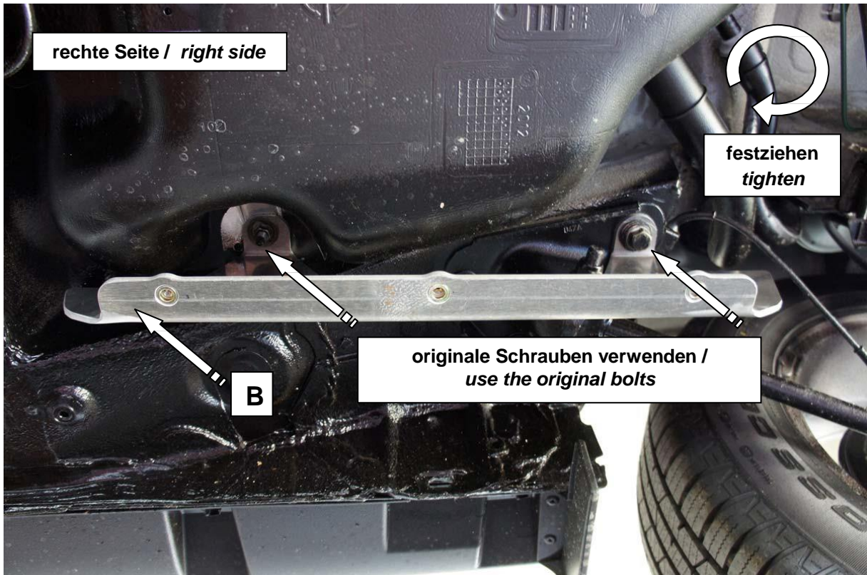
Konsole "B" anbringen / Attach bracket "B"
