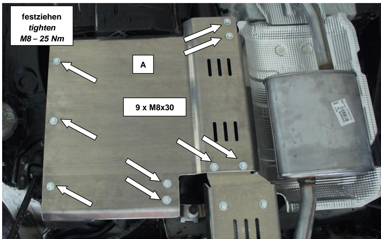
Schutzplatte "A" anbringen / Attach skid plate "A"
